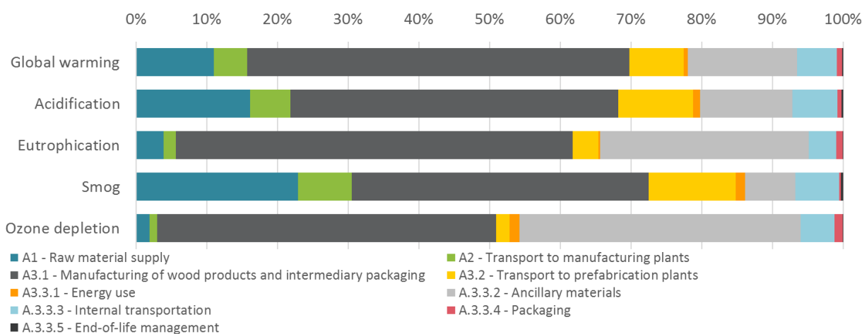
Figure 2: Relative contributions of the main processes in the production of prefabricated open walls
