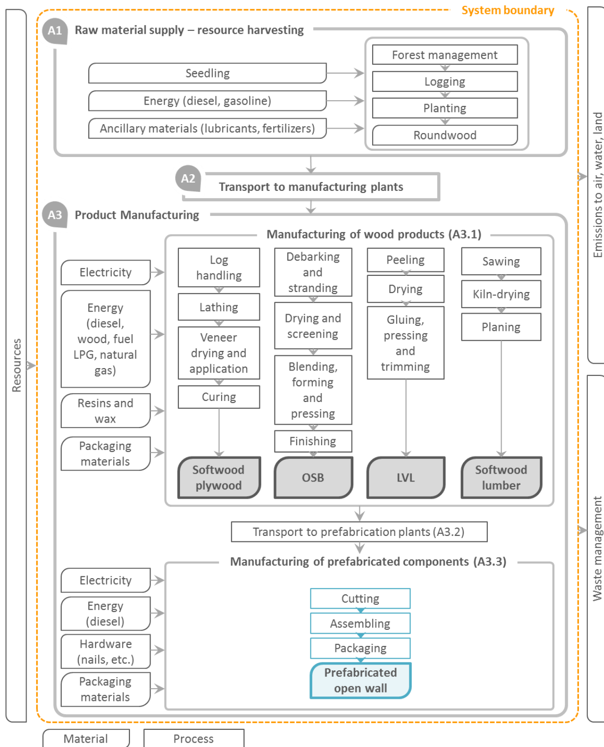
Figure 1: Process flow for manufacturing prefabricated open walls
